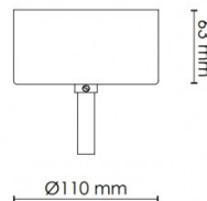
Ceiling Canopy (Model Ø110 x 63mm)
