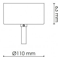
Ceiling Canopy (Model Ø110 x 63mm)
