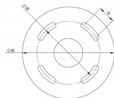
WALL PLATE
